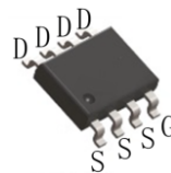
SOP-8 Top View
