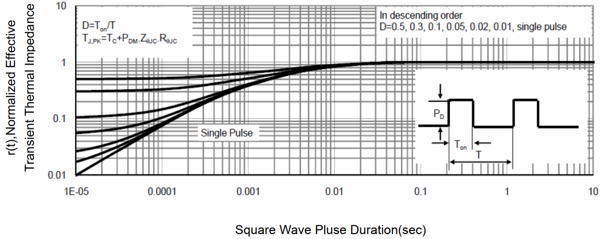
Figure 11b Normalized Maximum Transient Thermal Impedance (SOP-8)
