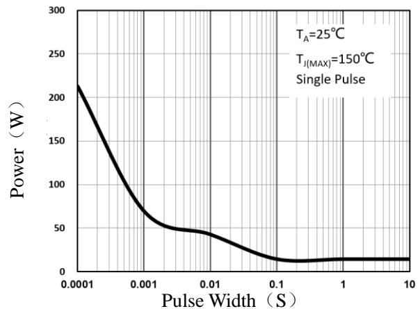
Figure 10b Single Pulse Power Rating Junction-to-Ambient (SOP-8)
