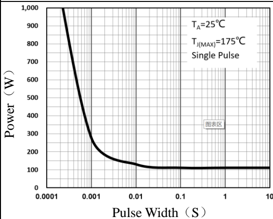
Figure 10a Single Pulse Power Rating Junction-to-Ambient (TO-220/252)
